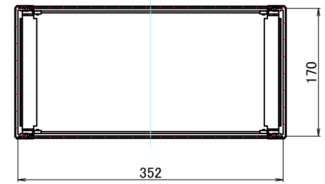
C-C (1:5)
