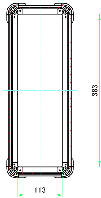
B-B (1:5.5)
