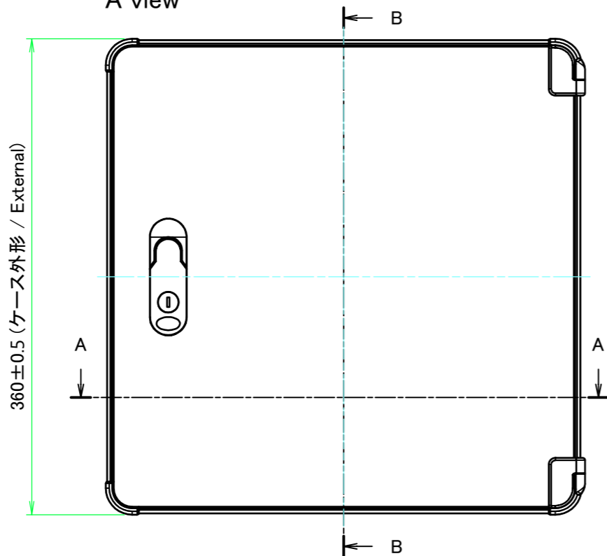
A view
