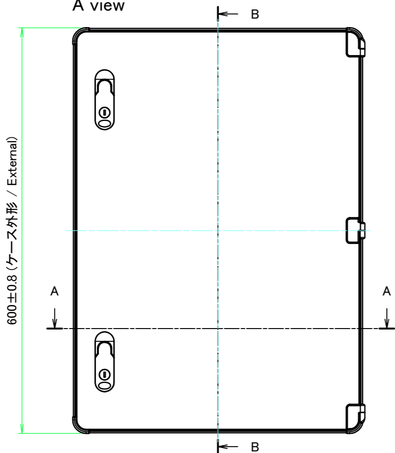
A view
