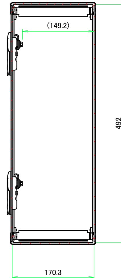
B-B (1:4.5)
