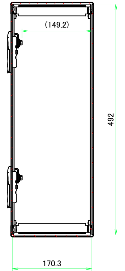
B-B (1:5)
