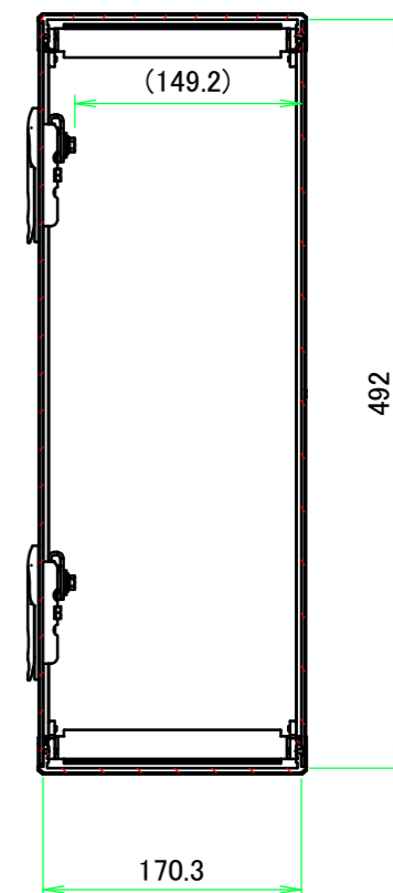
B-B (1:5.5)
