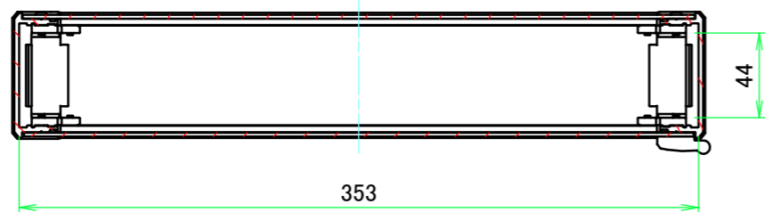
E view
