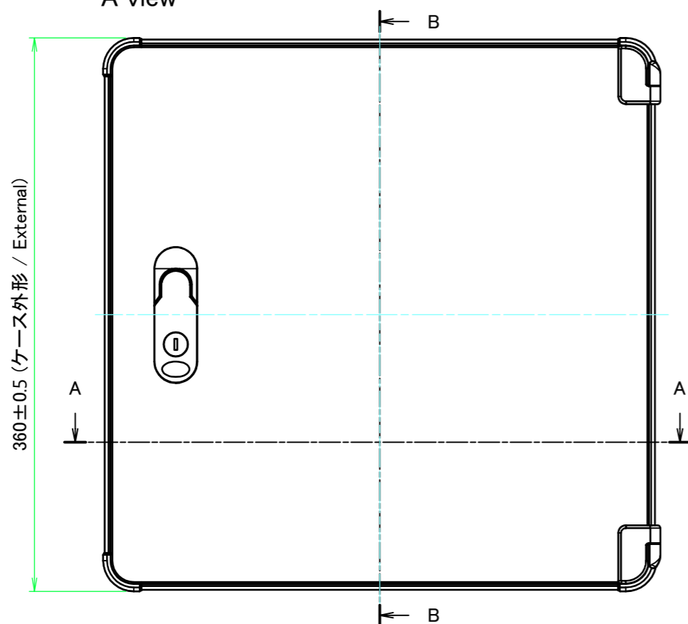
A view
