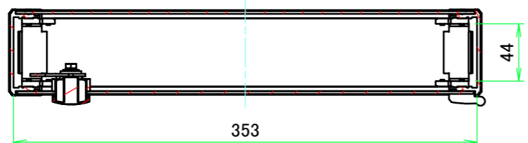
E view
