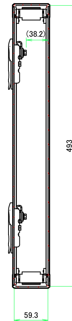
B-B (1:4)
