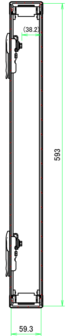
B-B (1:4.5)
