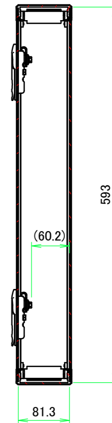
B-B (1:6)
