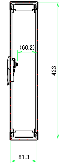
B-B (1:5.5)
