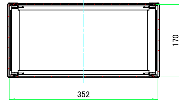
C-C ( 1 :5.5 )
