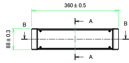
A view
