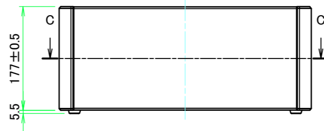
A view
