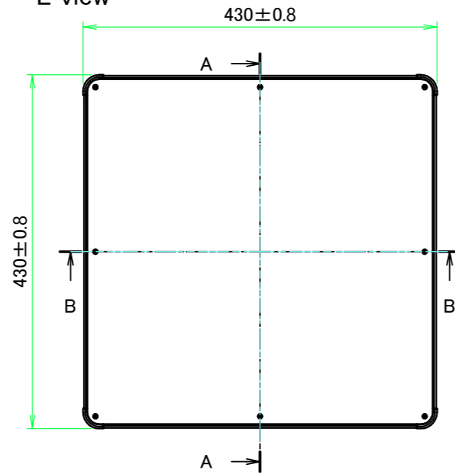
E view
