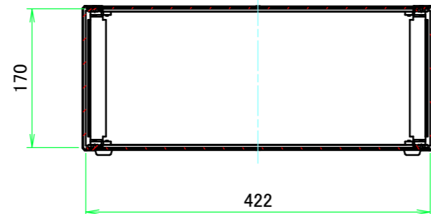
B-B (1:6.5)
