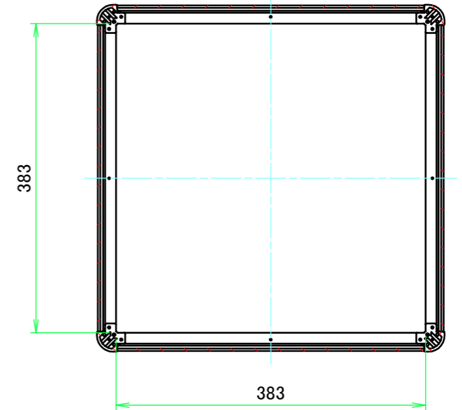
C-C (1:6.5)
