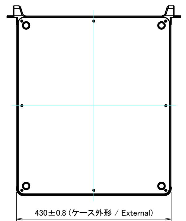
F view
