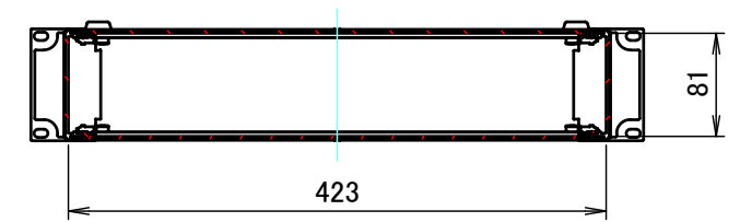
C-C (1:6.5)
