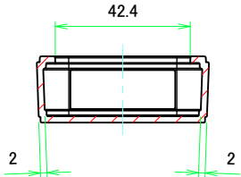
B-B (1:1.5)
