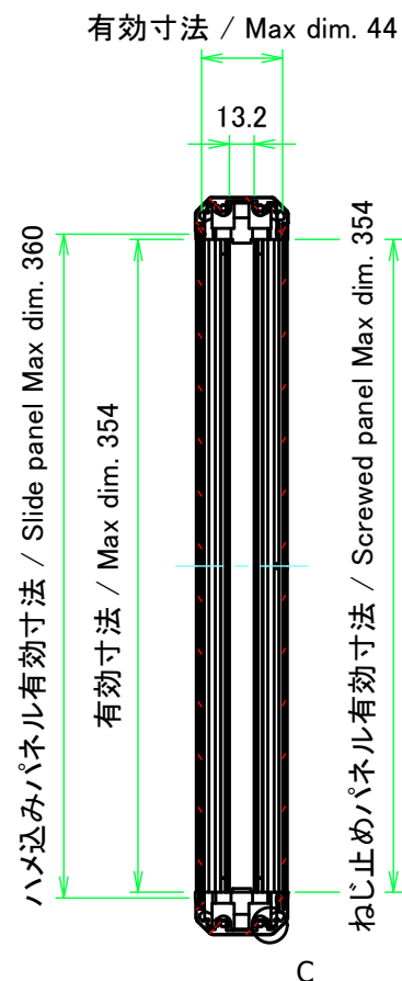
B-B (1:4.5)
