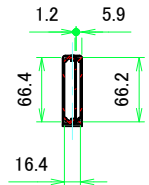
A-A (1:5.5)
