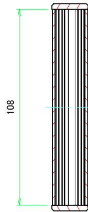
B-B (1:1.5)
