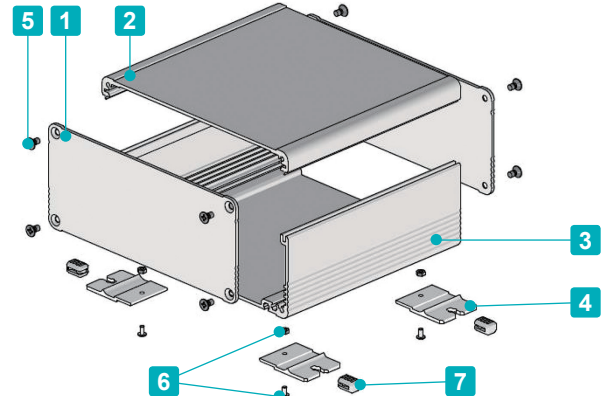
Flanged bracket type EXFS19-□, 23-□ and 29-□
