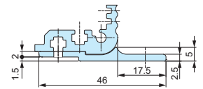
EXF • EXFS series Flange bracket dimensions (Section A)
